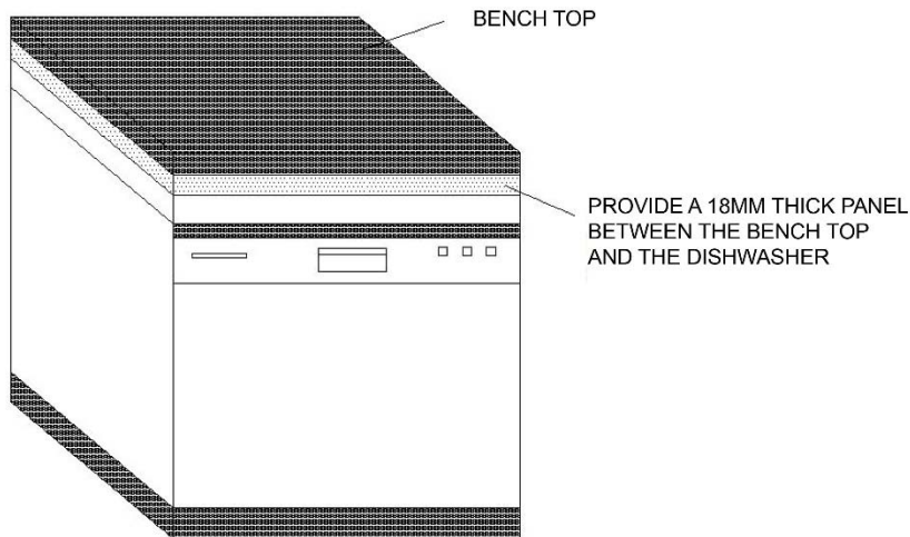
DISHWASHER INSTALLATION
